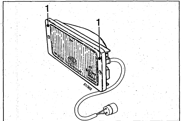
1 Adjusting screws for fog-light alignment, 9000 CD
