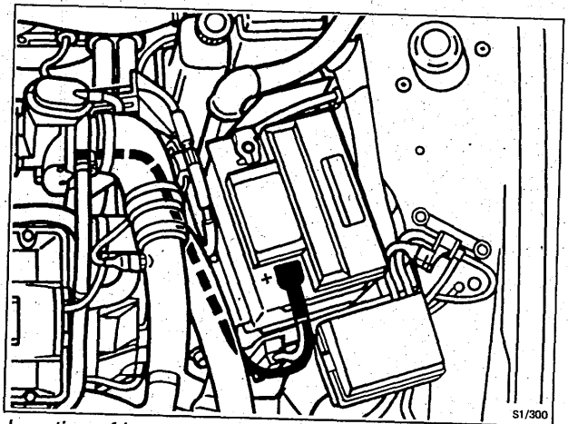
Location of battery, M1994
