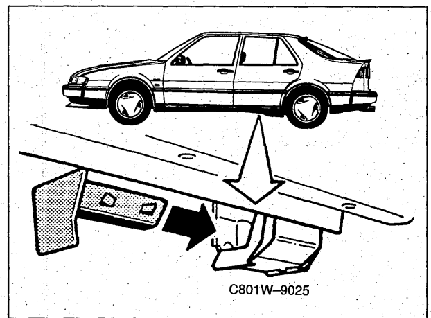
Fitting the stone chip guards
