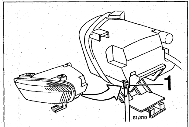
1 Adjusting screw for fog light alignment, 9000 CS
